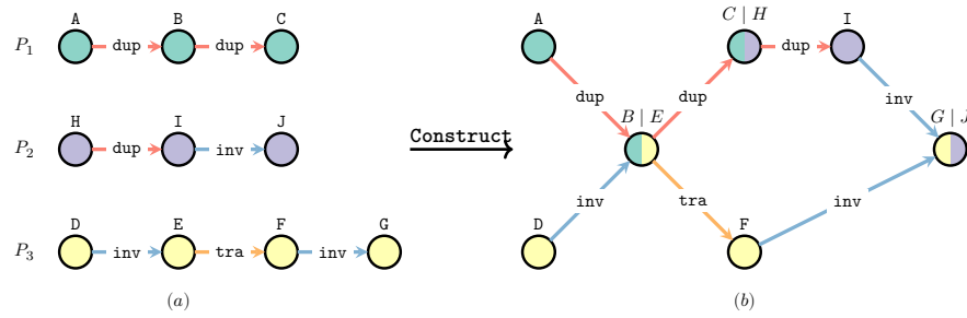
Figure 4: qual graph code
