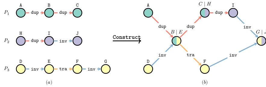
Figure 7: qual graph code
